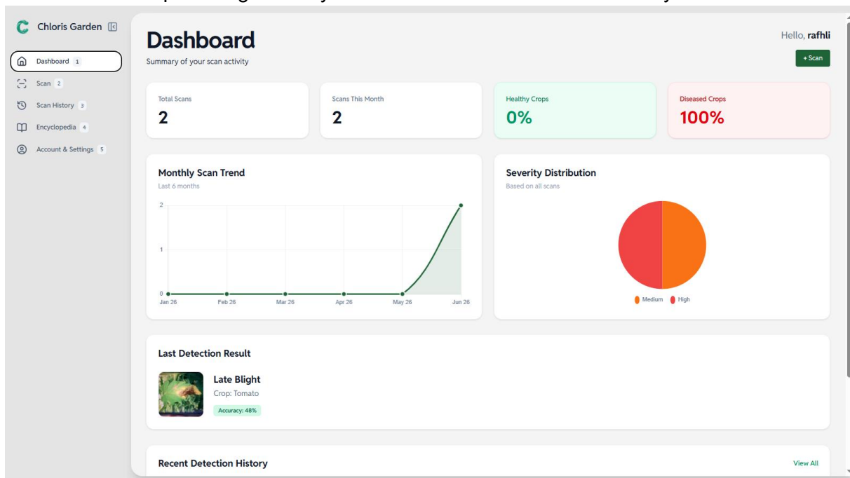
Gambar 12 Halaman Dashboard
